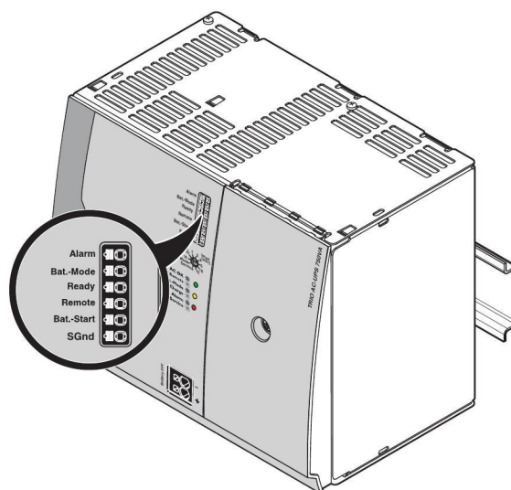
Figure 20 Signal outputs
