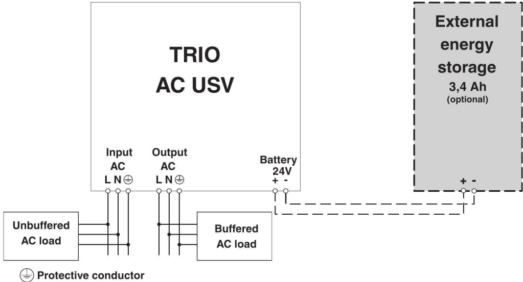
Figure 10 Schematic design
